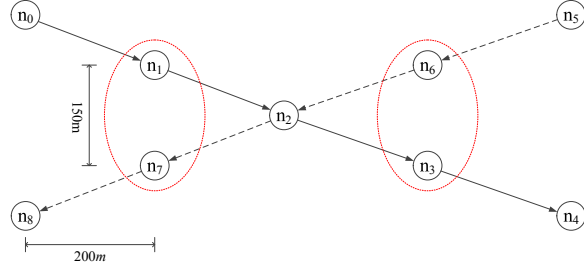
Fig. 6. X-II Topology
