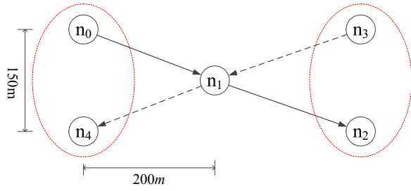
Fig. 4. X-I Topology
