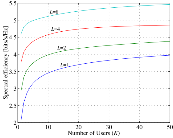
Fig. 1. Spectral efficiency at SINR 16 dB per receiver antenna, L th order MRC diversity in the mobile and K th order of selection diversity between the users.
